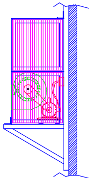
Wall Bracket
