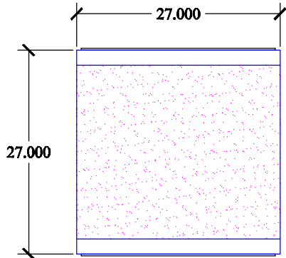
INLET VIEW
