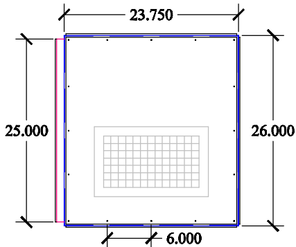
EXHAUST VIEW
